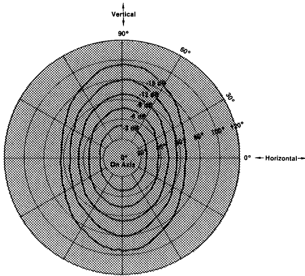
1 kHz octave bandwidth constant sound pressure contours of 0 to -15 dB in steps of -3 dB. The contours are plotted on polar grid lines with on axis being the center of the plot. The data was gathered by taking an octave polar plot at all oblique angles from 0° (horizontal) to 90° (vertical) in steps of 15°. Same test conditions as horizontal polar response.
