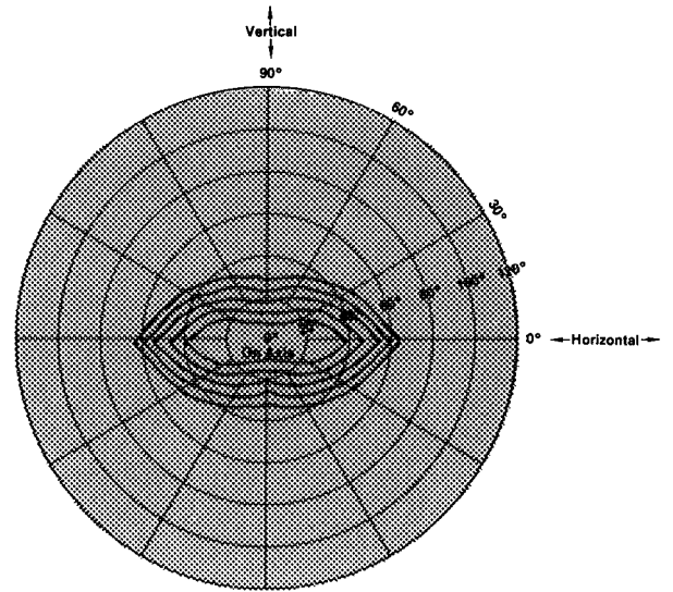
8 kHz octave bandwidth constant sound pressure contours. Same conditions as 1 kHz contours.
